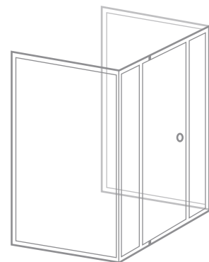
5P2S Five panels, one door, two infills, two squared returns, optional stabilising shelf return
